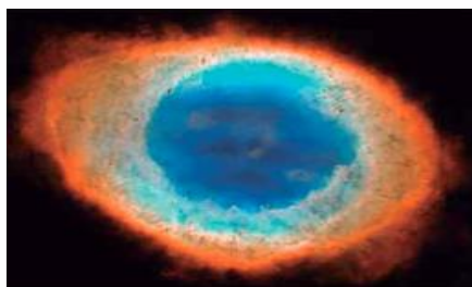
Nebulosa do Anel
